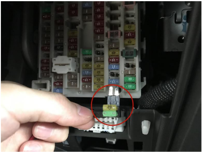
Then insert our power plug to original fuse port per picture
